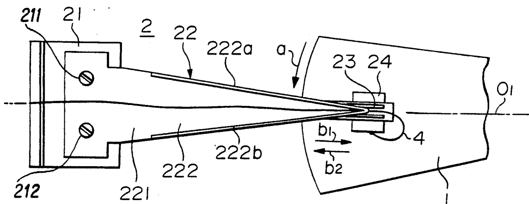
FIGURE 6 PRIOR ART
