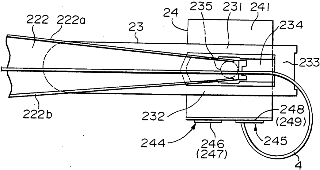
FIGURE 8 PRIOR ART
