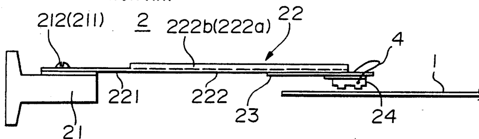
FIGURE 7 PRIOR ART
