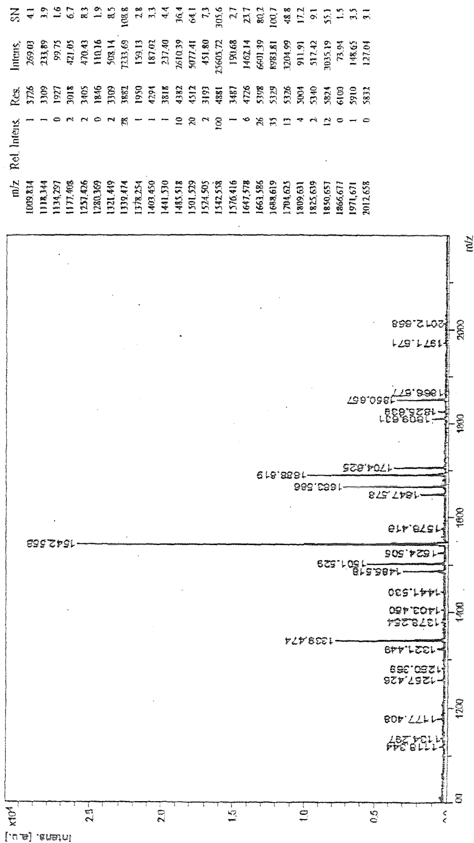
MALDI/TOF-MS oligosaccharide profile for glycoengineered humanized anti-EGFR IgG1 antibody IHHB-KC.
