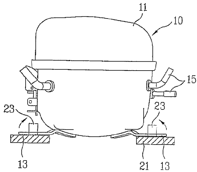
FIG. 3 Prior Art
