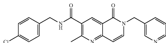
N-(4-chlorobenzyl)-2-methyl-5-oxo-6-(pyridin-3-ylmethyl)-5,6-dihydro-1,6-naphthyridine-3-carboxamide
