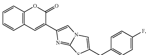
3-(2-(4-fluorobenzyl)imidazo[2,1-b]thiazol-6-yl)-2H-chromen-2-one
