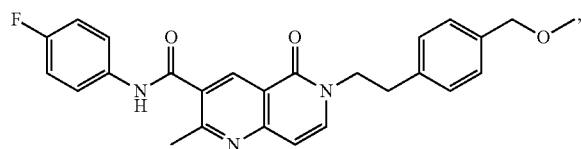
N-(4-fluorophenyl)-6-(4-(methoxymethyl)phenethyl)-2-methyl-5-oxo-5,6-dihydro-1,6-naphthyridine-3-carboxamide
