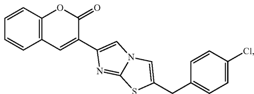
3-(2-(4-chlorobenzyl)imidazo[2,1-b]thiazol-6-yl)-2H-chromen-2-one
