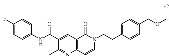
N-(4-fluorophenyl)-6-(4-(methoxymethyl)phenethyl)-2-methyl-5-oxo-5,6-dihydro-1,6-naphthyridine-3-carboxamide
