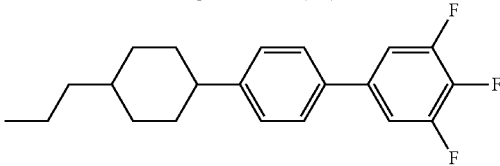
Example 4. 3-HBB(F,F)-F
