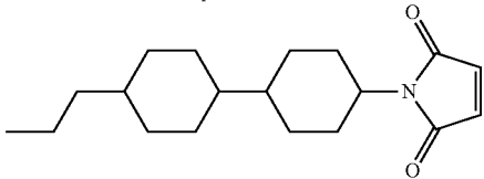
Example 2. 5-HHBB(F,F)-F
