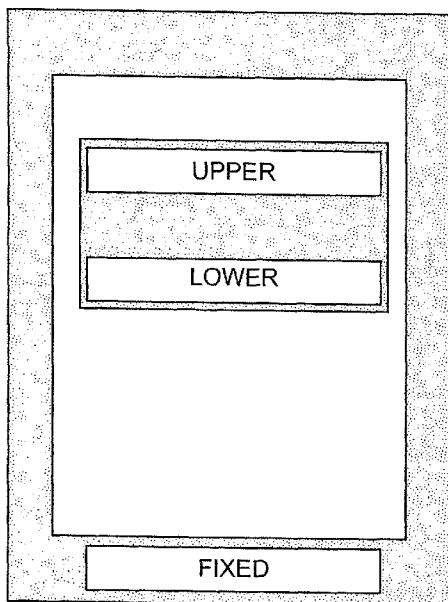
CROSS-SECTION SHOWING MEMS BEAM (UPPER AND LOWER ELECTRODES WITH SiO 2 BETWEEN THEM, ON SIDES, AND OVER/UNDER)
