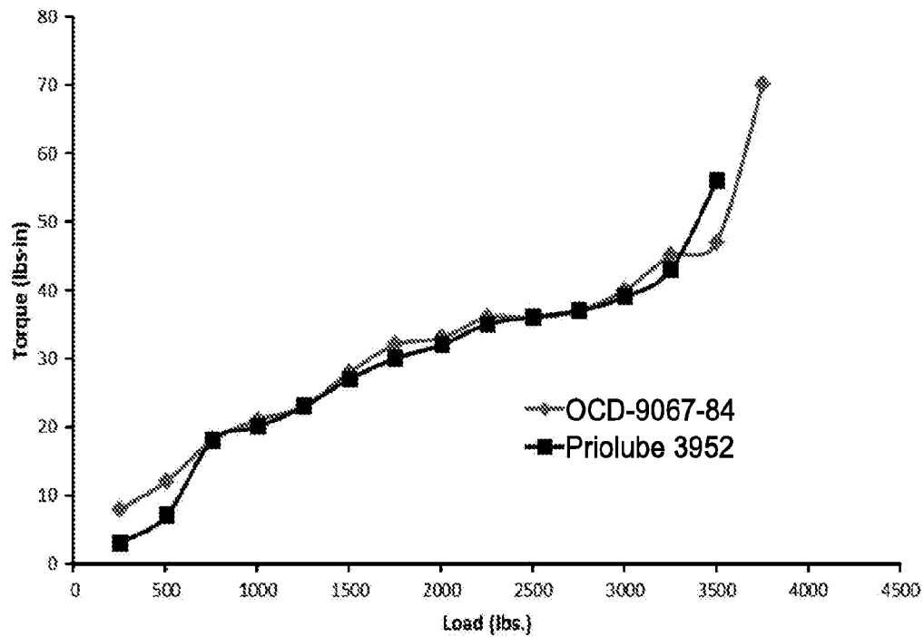
FIG. 14 Torque Difference Between Samples A & B in 300 ppm Hard Water
