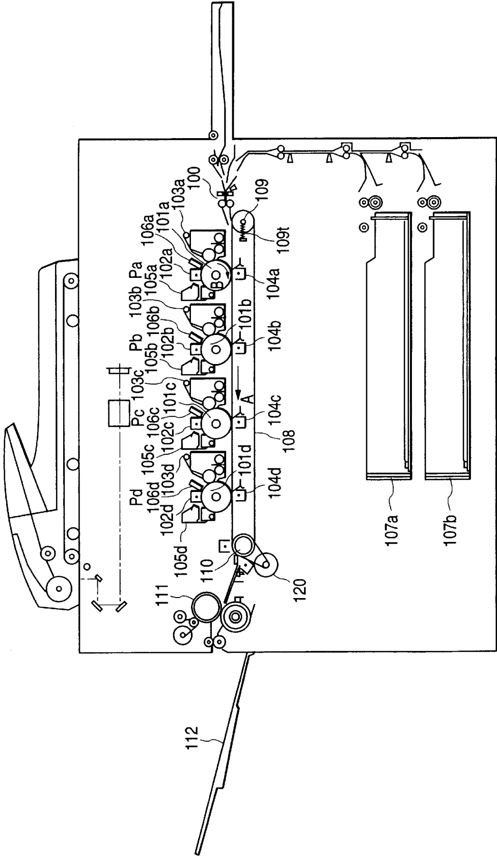
FIG. 23 PRIOR ART
