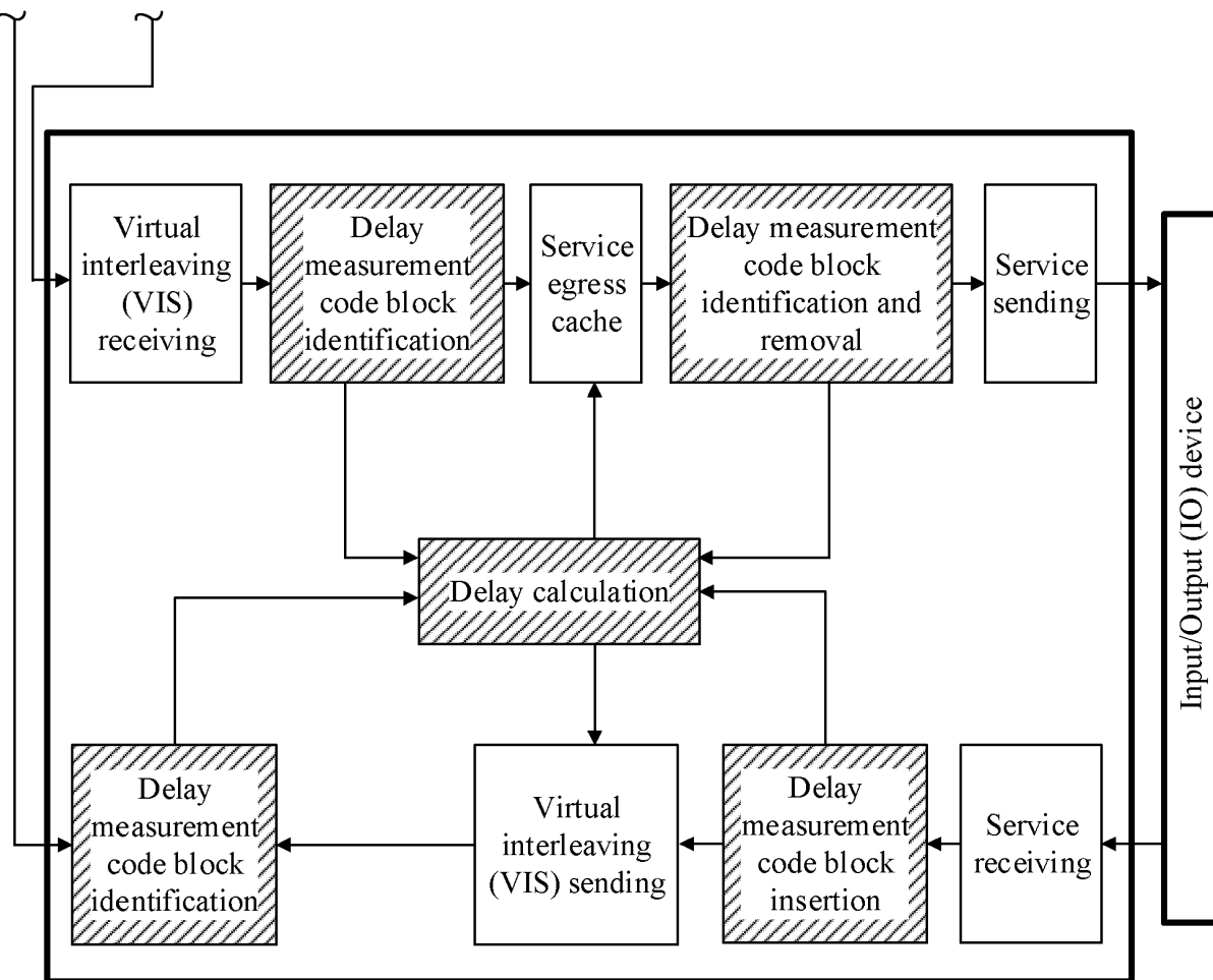
Third switch device (VIS 3)-Edge device
