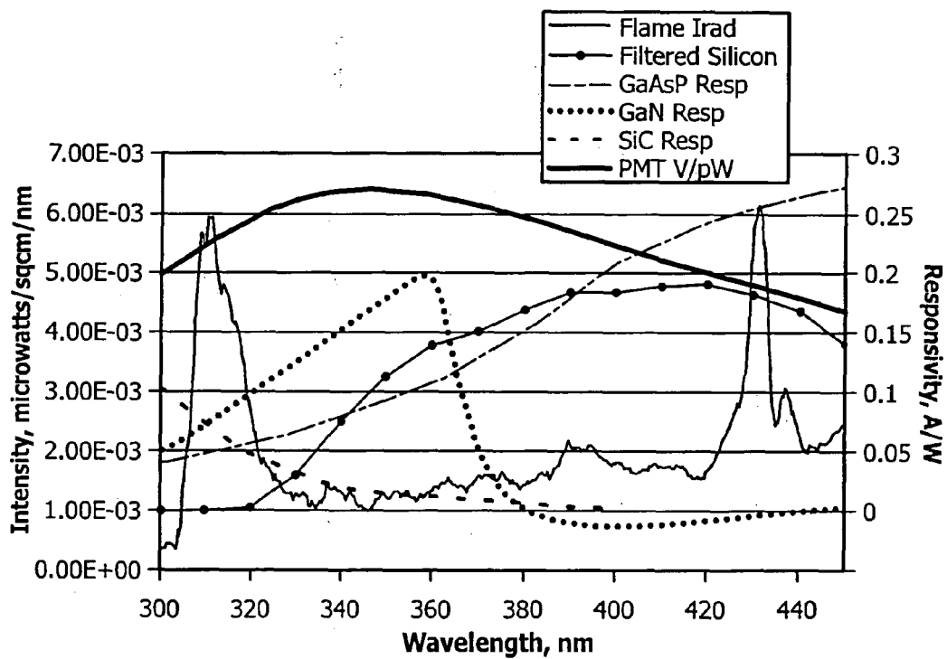
Flame Spectrum vs Photodiode Responsivity
