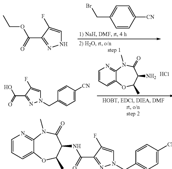
Step 1: Preparation of 1-(4-cyanobenzyl)-4-fluoro-1H-pyrazole-3-carboxylic acid
