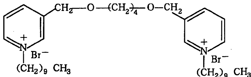
Compound (7-C)
