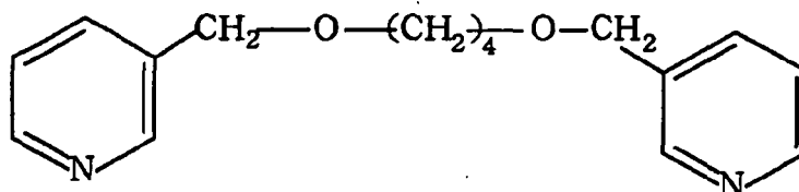
Compound (5-A)
