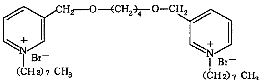
Compound (7-A)
