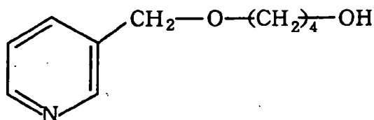
Compound (3-A)
