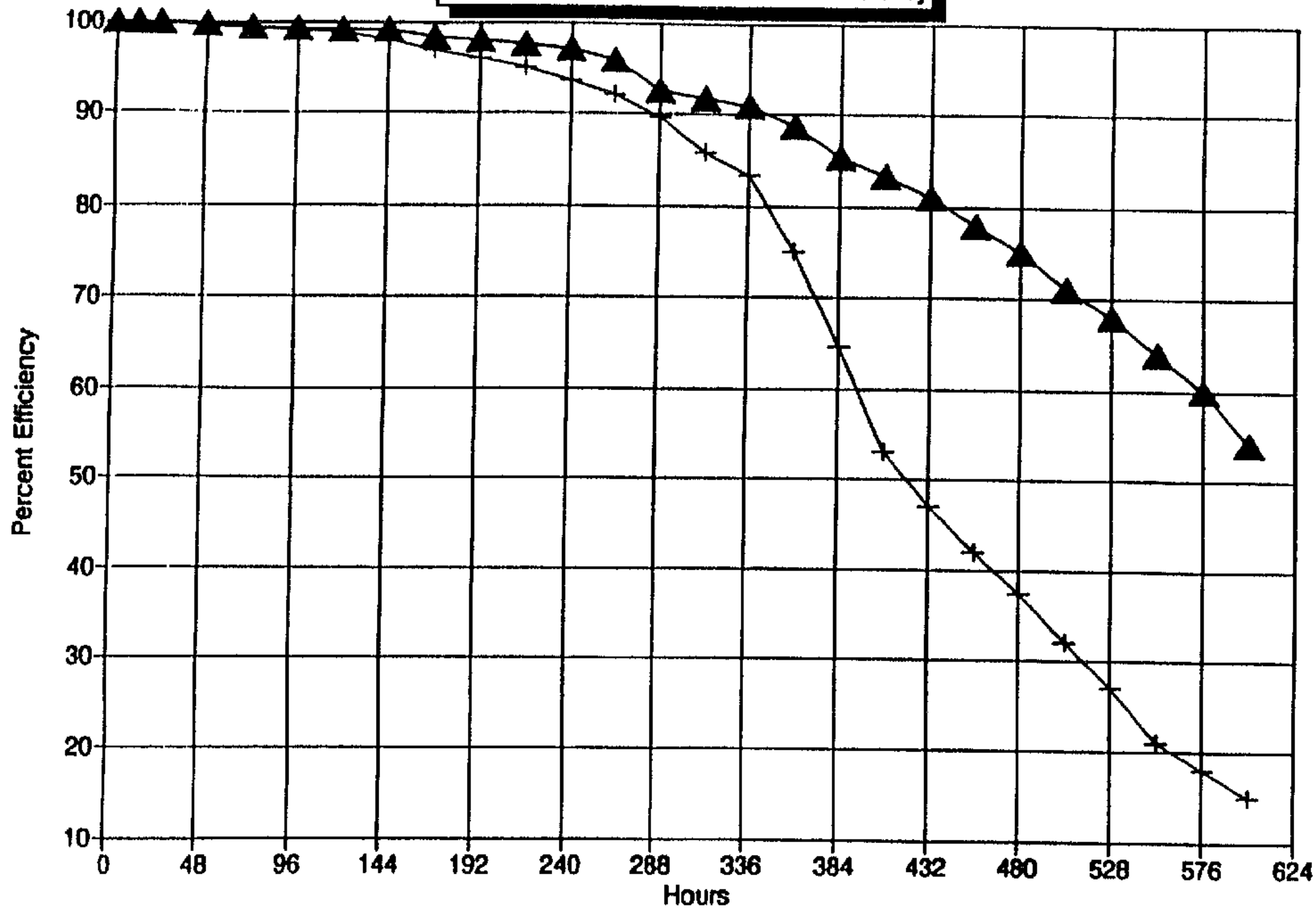
4% & 8% KMnO4 vs H2S Removal Efficiency
