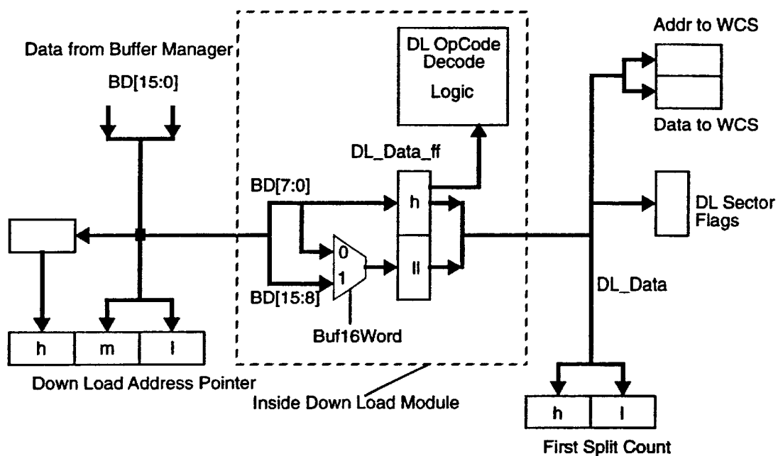
Down Load Module Data Path Diagram
