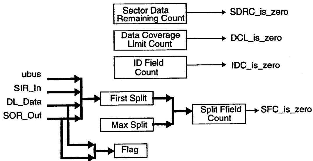
INTER-FIELD LOGIC BLOCK DIAGRAM
