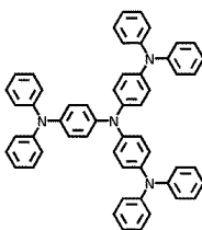
TDATA
