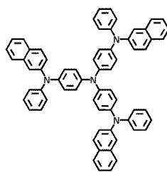
2-TNATA
