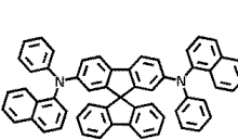
Spiro-NPB
