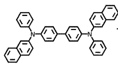
β-NPB
