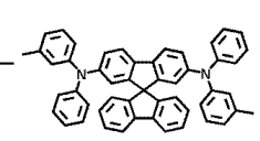
Spiro-TPD
