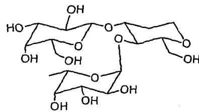
Compound B
