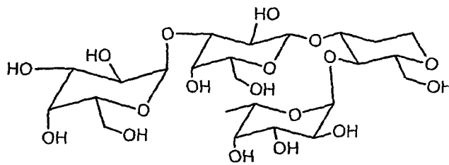
Glycomimetic 1
