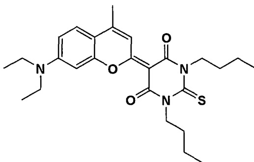
Spectral sensitizing dye d-0
