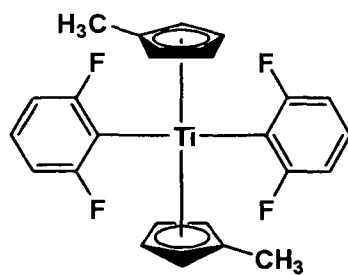
Organometallic compound a
