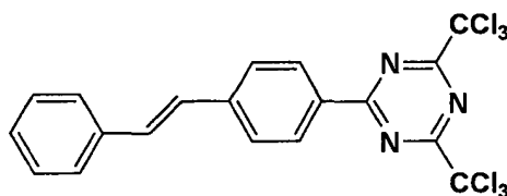
Spectral sensitizing dye d-0
