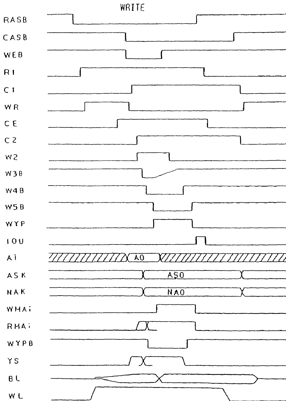
FIG. 76 CAS SYSTEM (WRITE OPERATION)
