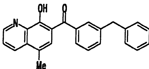
Compound [C]
