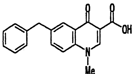
Compound [G]
