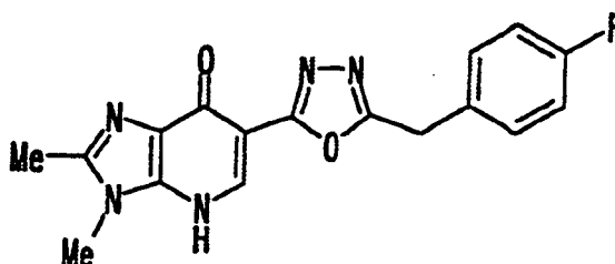
Compound [B]
