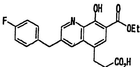
Compound [A]
