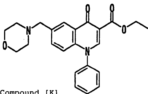
Compound [K]
