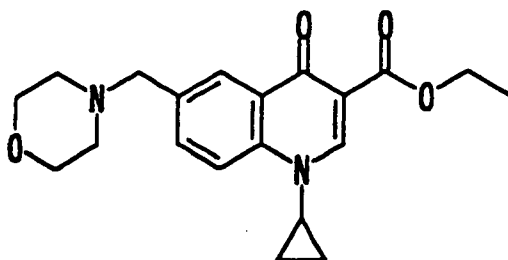
Compound [H]
