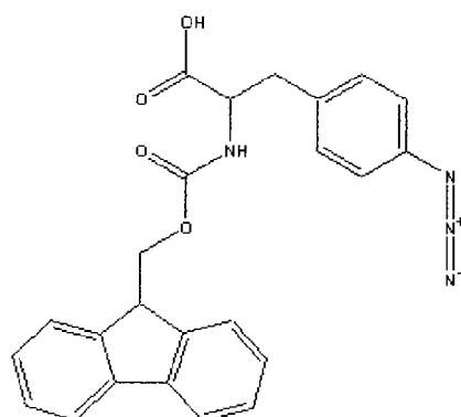
Fmoc-4-azidophenylalanine
