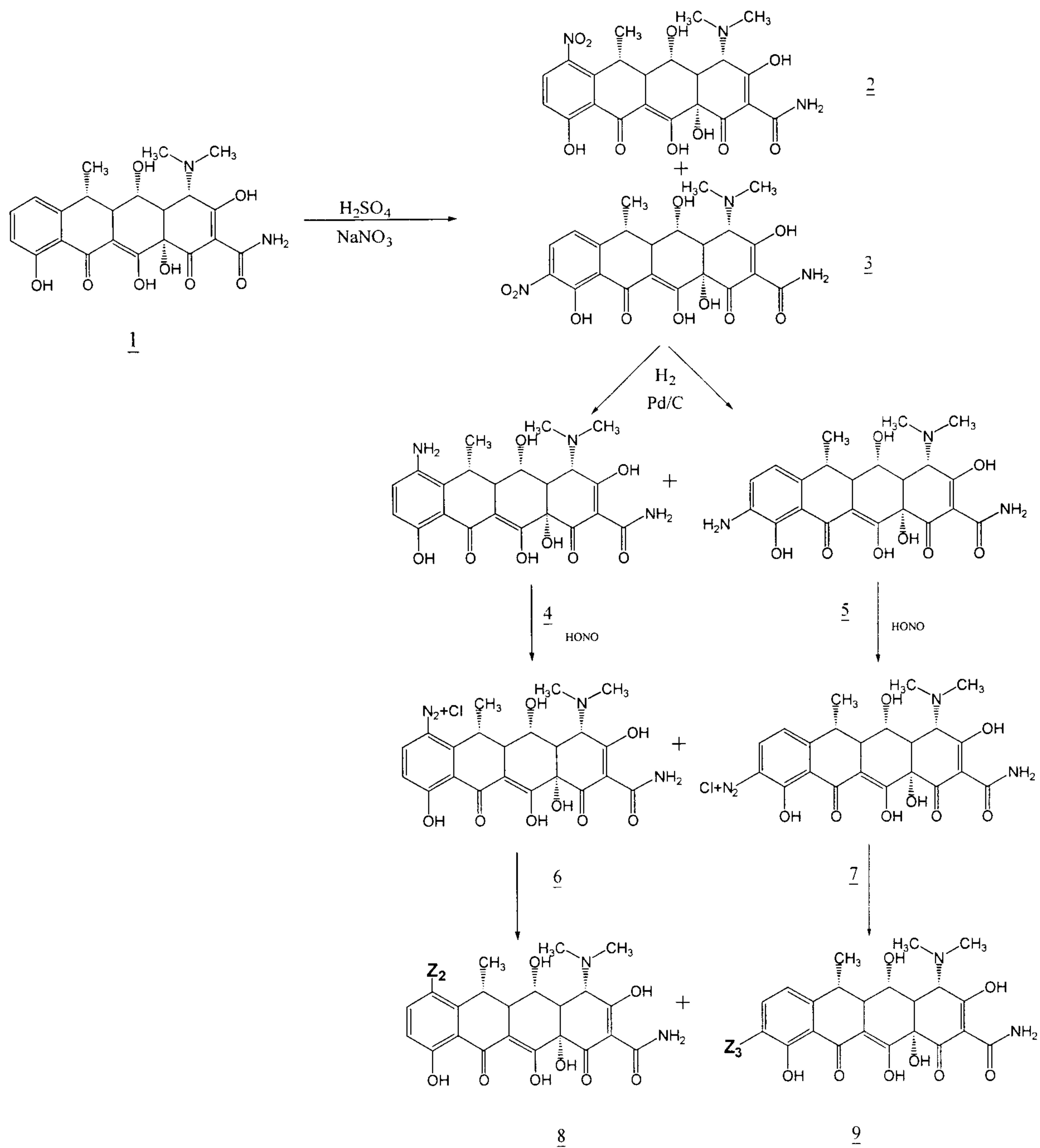
Scheme I
