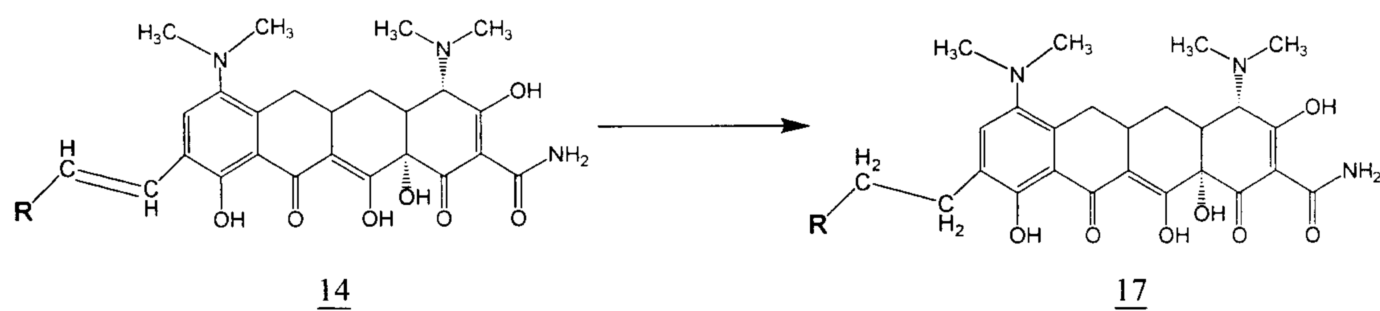
Scheme V
