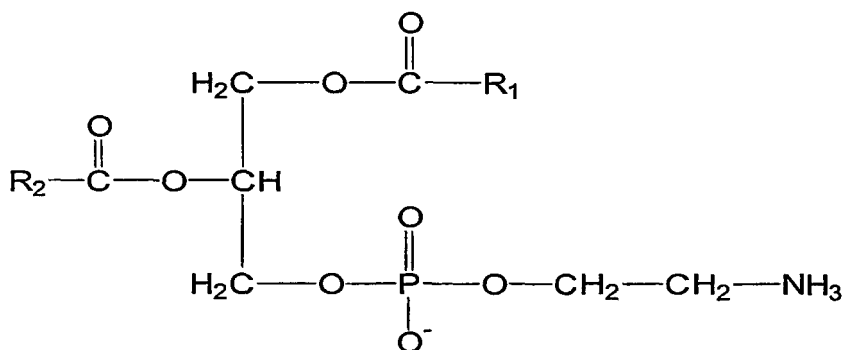
Phosphatidylethanolamine— common structure \text{R}_1 and \text{R}_2 are fatty acid residues, different for each molecular species
