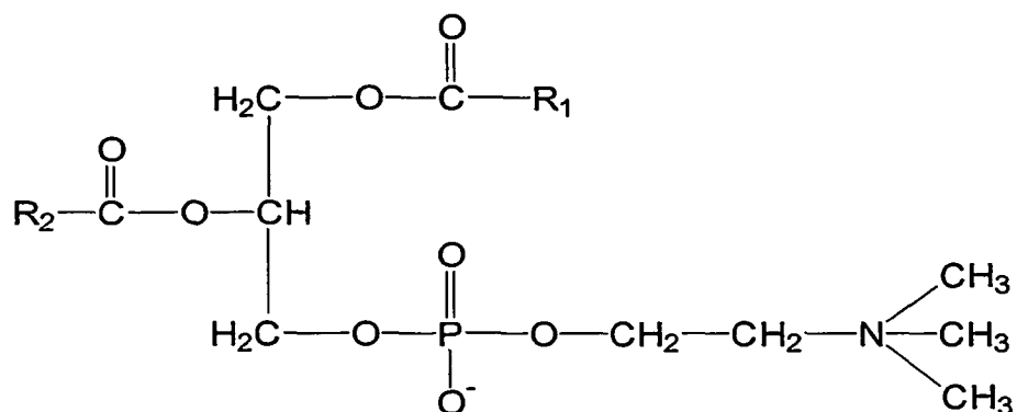
Phosphatidylcholine — common structure \text{R}_1 and \text{R}_2 are fatty acid residues, different for each molecular species
