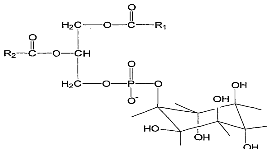
Phosphatidylinositol— common structure R 1 and R 2 are fatty acid residues, different for each molecular species
