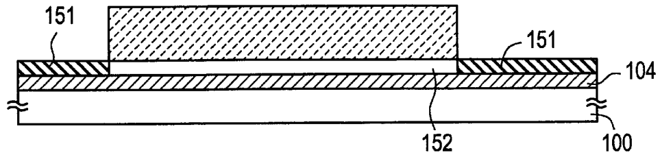
FIG.11B STEP OF ADDING PHOSPHORUS
