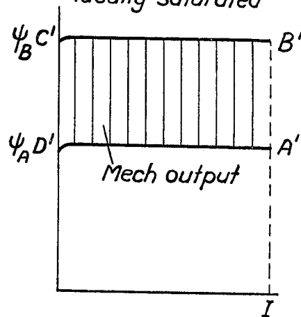
Fig. 10 Ideally saturated
