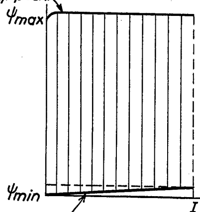
Fig. 12 Ideally saturated
