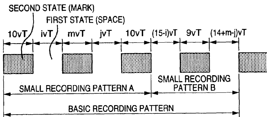
EMBODIMENT 1 OF BASIC RECORDING PATTERN
