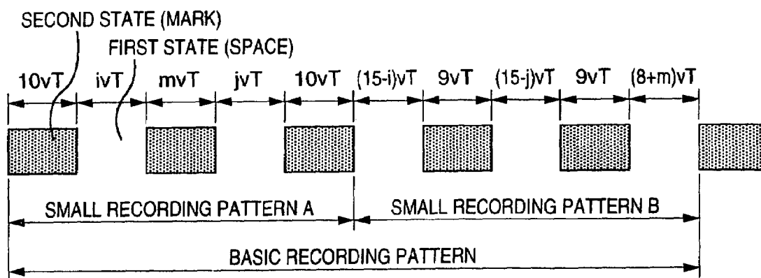
EMBODIMENT 2 OF BASIC RECORDING PATTERN
