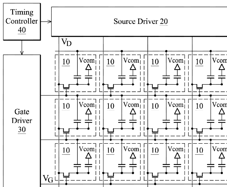
FIG. 1 (RELATED ART)
