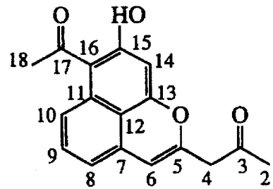
RM 18 (10)
