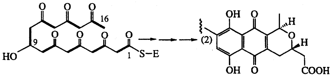
ACTINORHODIN (3)
