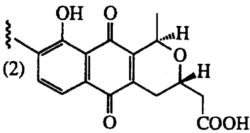
ACTINORHODIN (3)
