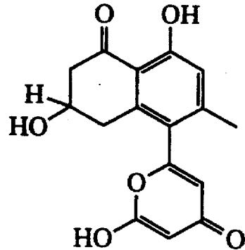
MUTACTIN (6)
