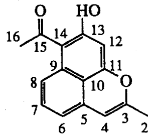
RM 18b (11)
