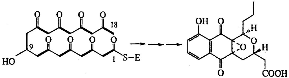
FRENOLICIN B (7)
