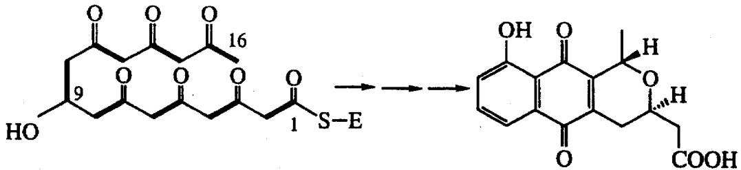
NANAOMYCIN A (8)
