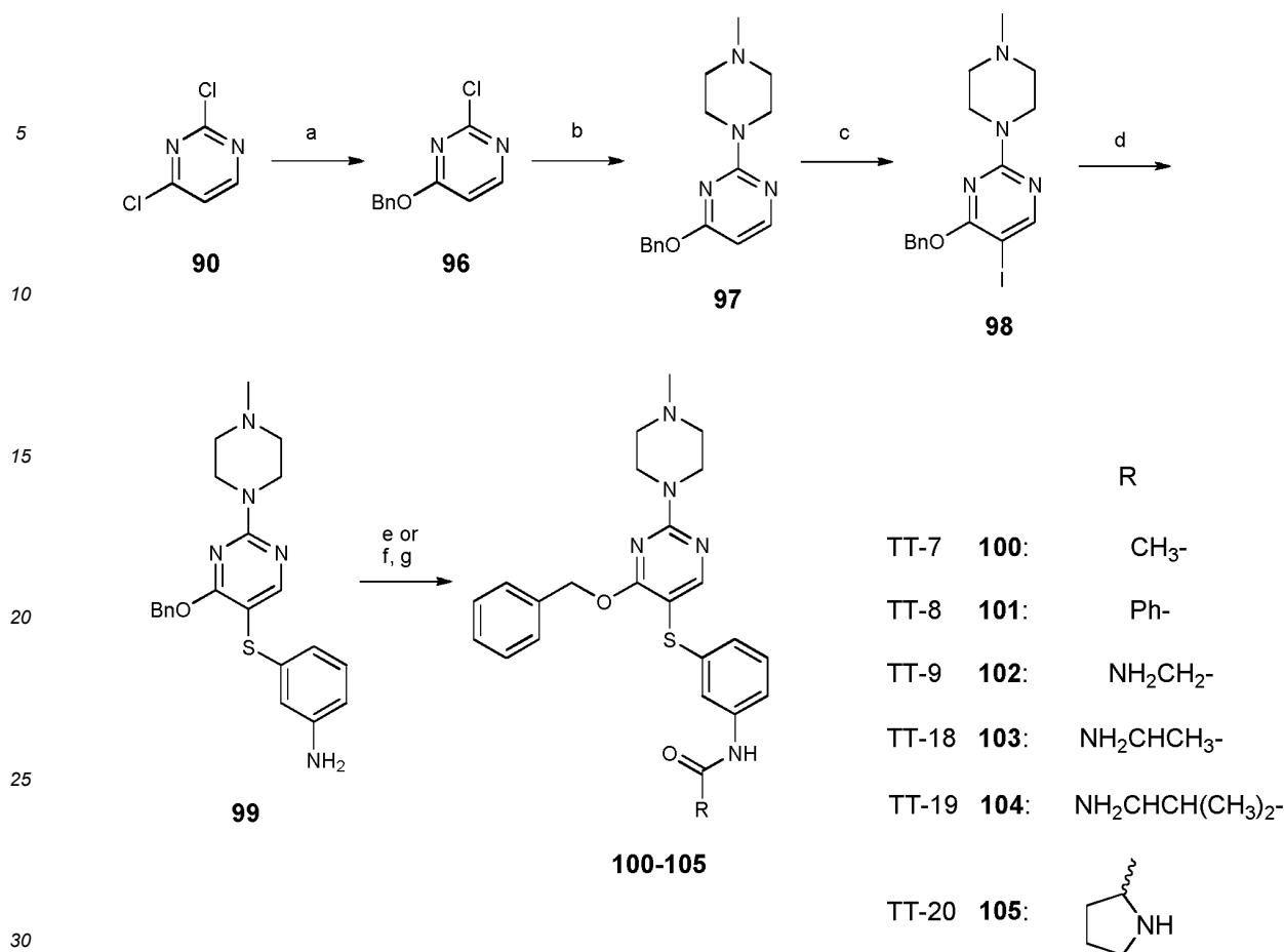
Scheme 12. Synthesis of TT-7 ( 100 ), TT-8 ( 101 ), TT-9 ( 102 ), TT-18 ( 103 ), TT-19 ( 104 ), TT-20 ( 105 ).
