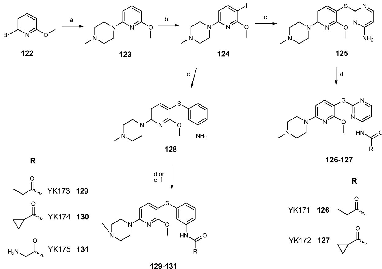
Scheme 15. Synthesis of YK171 ( 126 ), YK172 ( 127 ), YK173 ( 129 ), YK174 ( 130 ), YK175 ( 131 ).
