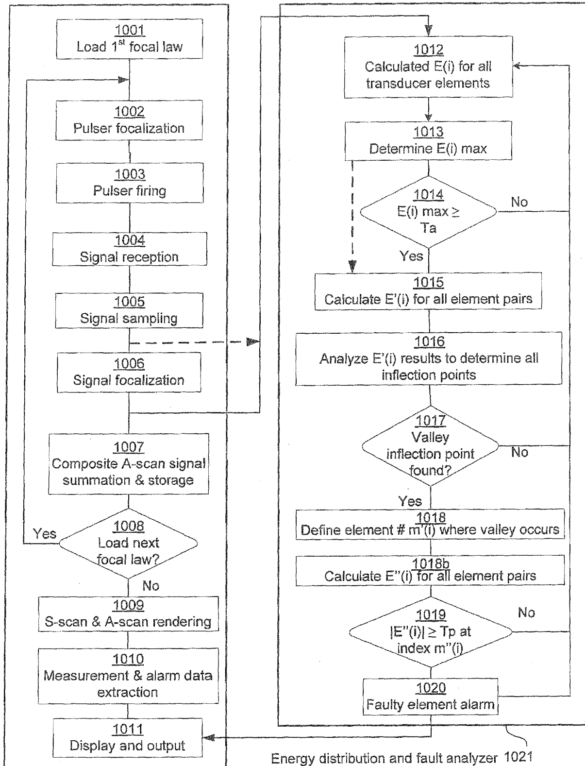
1000 Typical phased array instrument operating sequence
