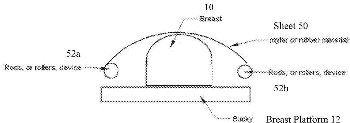
Compression system utilizing material stretched between two rods
