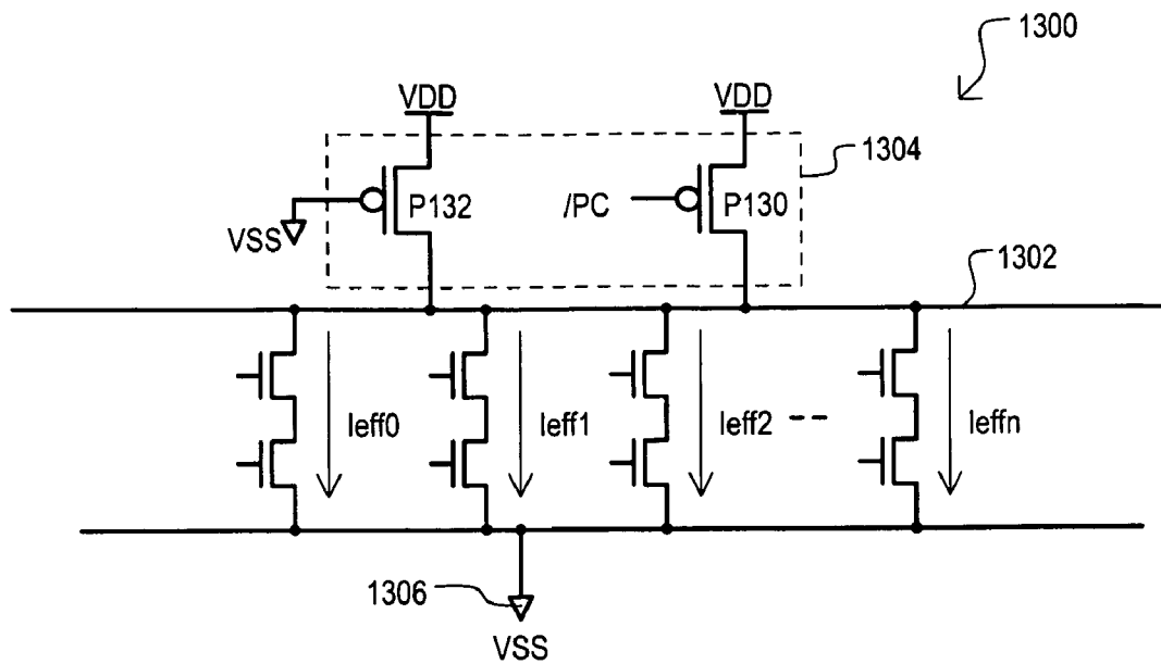
FIG. 13 (BACKGROUND ART)
