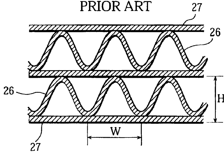
Fig. 12 PRIOR ART
