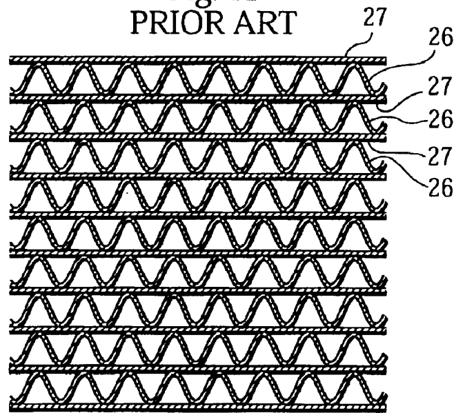
Fig. 13 PRIOR ART
