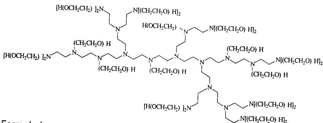
Formula I
