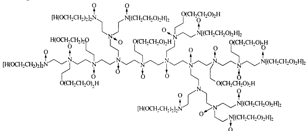
Formula II
