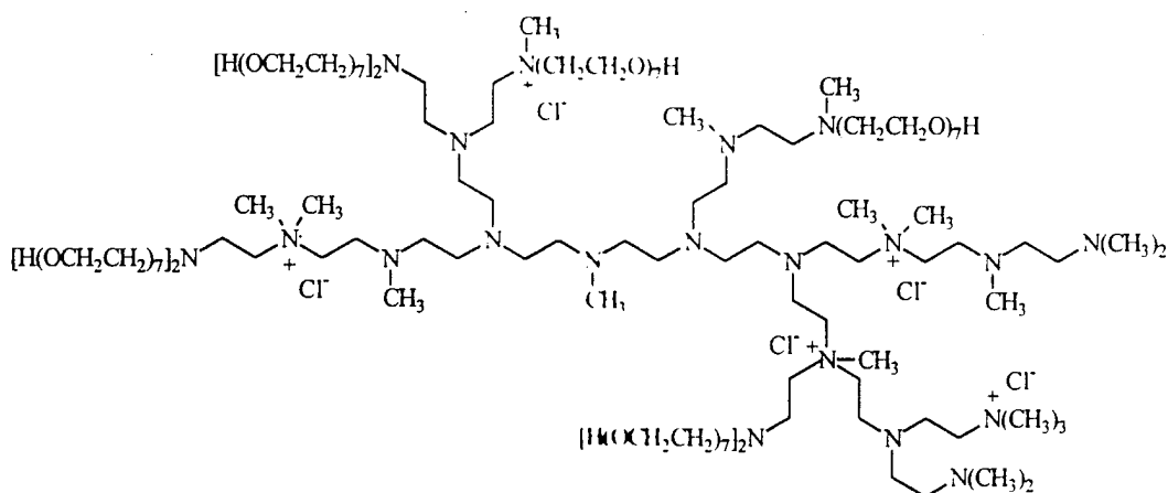
Formula III
