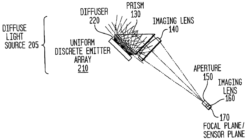
FIG. 2 (PRIOR ART) DIFF ONLY
