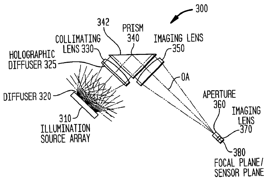
FIG. 3A INVENTION HYBRID ILLUM.
