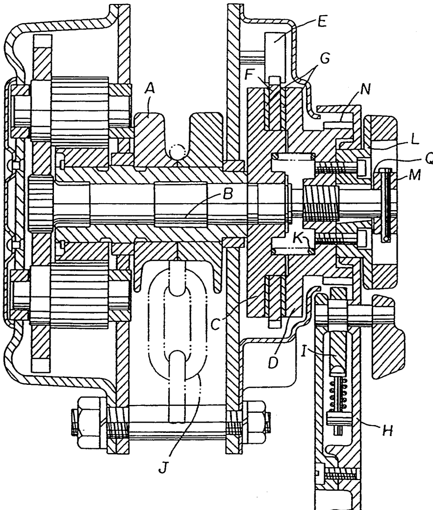
FIG. 14 (PRIOR ART)
