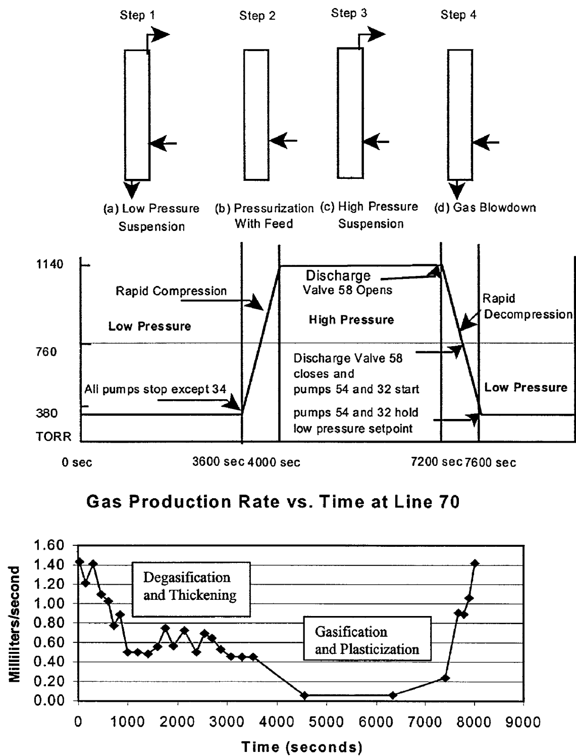
Fig 3. TAP Stage II: Simple Pressure Swing Cycle
