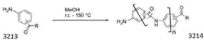
Reaction 2b
