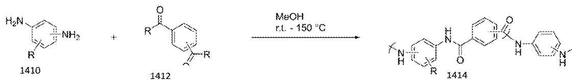
Reaction 1
