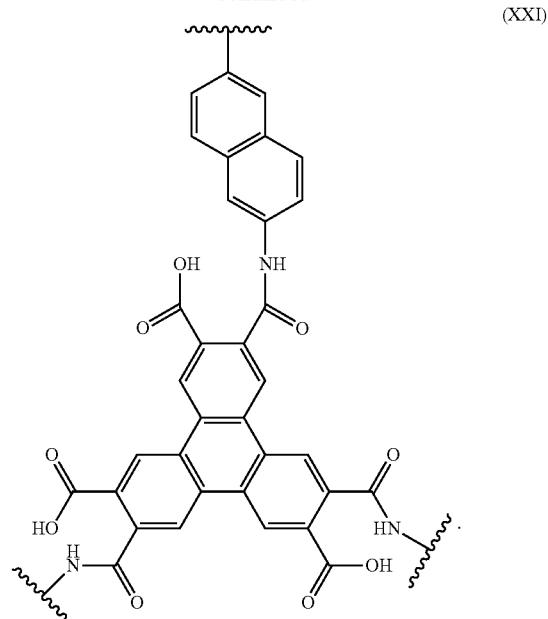
(XXI)
