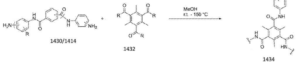
Reaction 3
