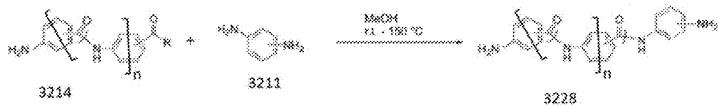
Reaction 2b
