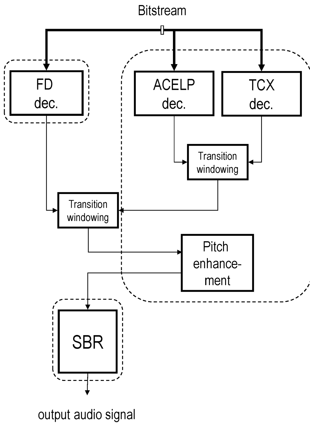
Fig. 6 (prior art)
