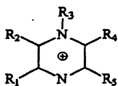
Pyrazinium
