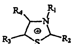
Thiazolium
