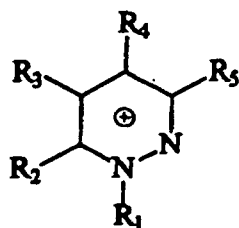
Pyridazinium
