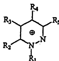
Pyridazinium
