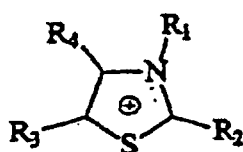
Thiazolium
