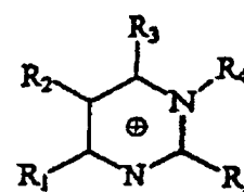
Pyrimidinium
