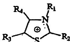
Thiazolium
