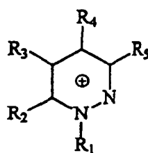
Pyridazinium
