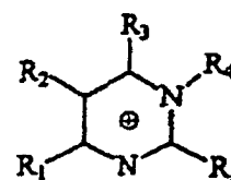
Pyrimidinium
