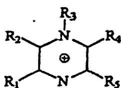
Pyrazinium
