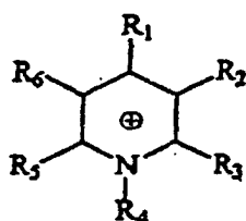
Pyridinium
