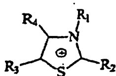
Thiazolium
