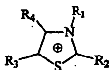
Thiazolium
