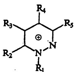
Pyridazinium
