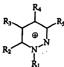
Pyridazinium
