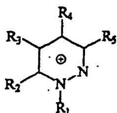
Pyridazinium
