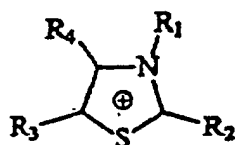
Thiazolium
