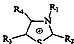
Thiazolium
