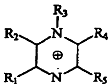
Pyrazinium
