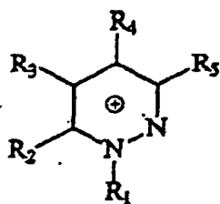
Pyridazinium
