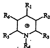
Pyridinium
