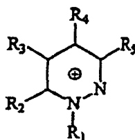
Pyridazinium
