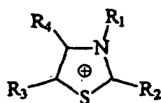
Thiazolium
