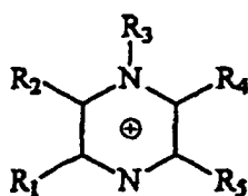
Pyrazinium
