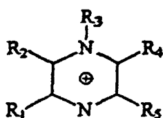
Pyrazinium
