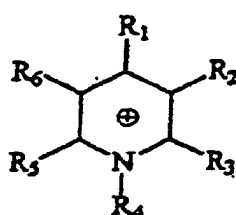
Pyridinium
