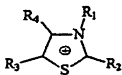
Thiazolium
