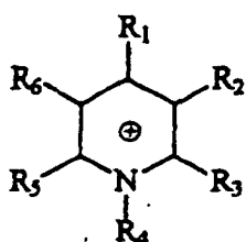
Pyridinium
