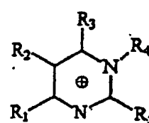
Pyrimidinium
