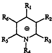
Pyridinium
