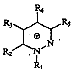
Pyridazinium
