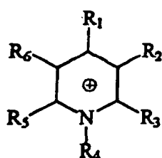
Pyridinium
