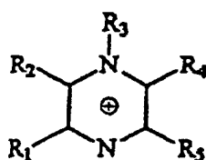
Pyrazinium
