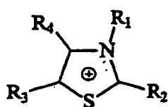
Thiazolium
