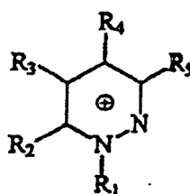
Pyridazinium
