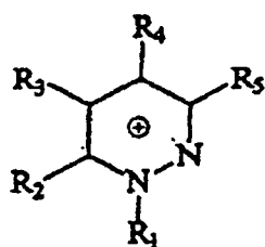
Pyridazinium
