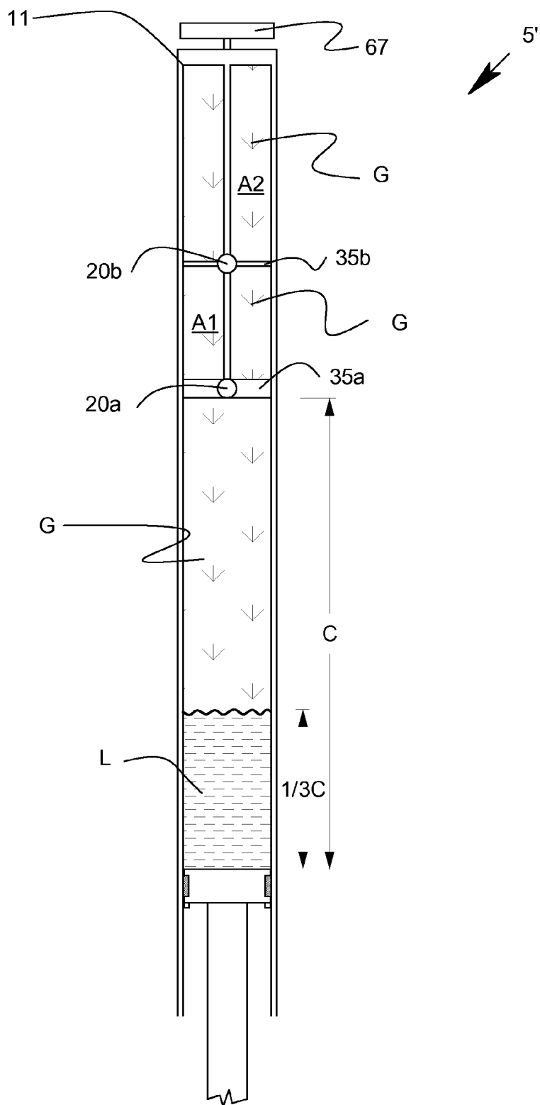
FIG 6 (Two Auxiliary Chambers)
