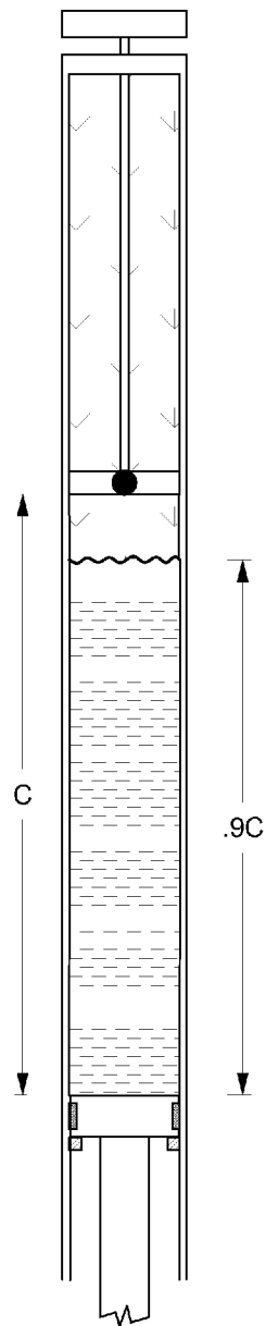
FIG 5D Substantially No Short Travel
