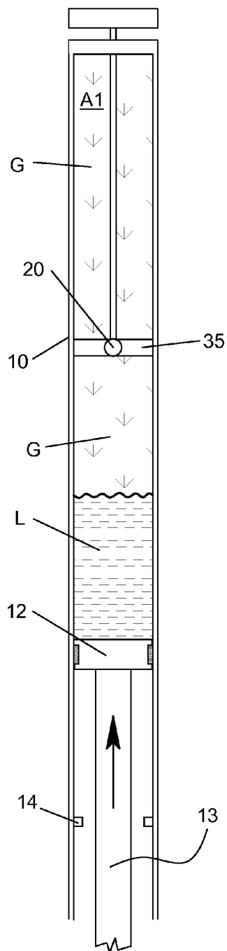
FIG 2A (Long Travel)
