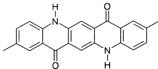
Pigment PR 122 (2,9-dimethylquinacridone)
