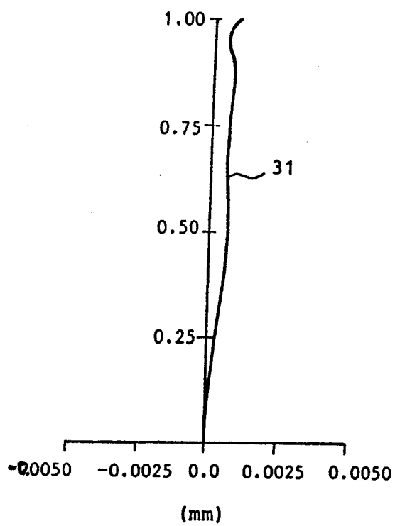
SPHERICAL ABERRATION
