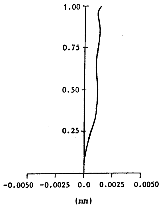
SPHERICAL ABERRATION
