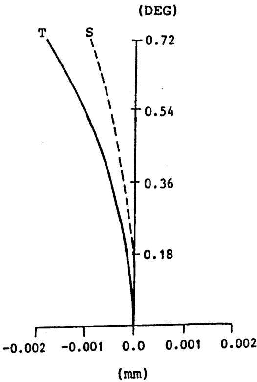
ASTIGMATISM
