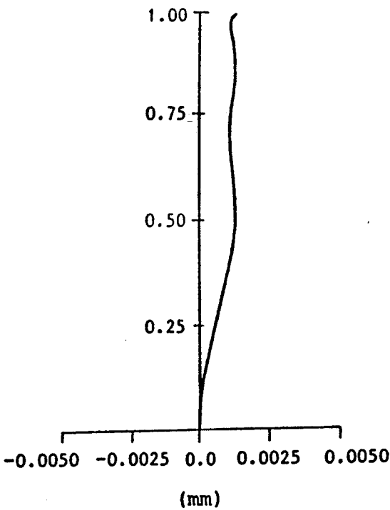
SPHERICAL ABERRATION
