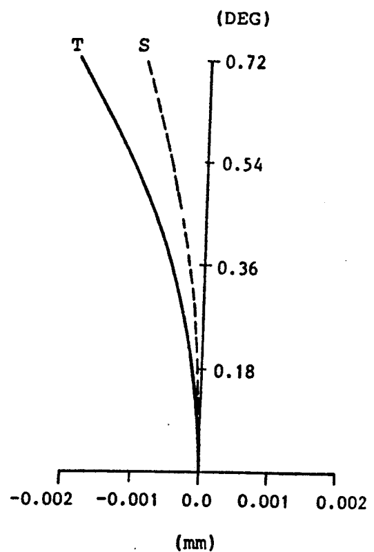
ASTIGMATISM
