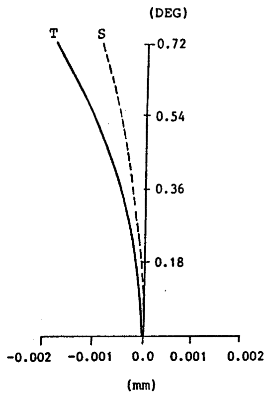
ASTIGMATISM
