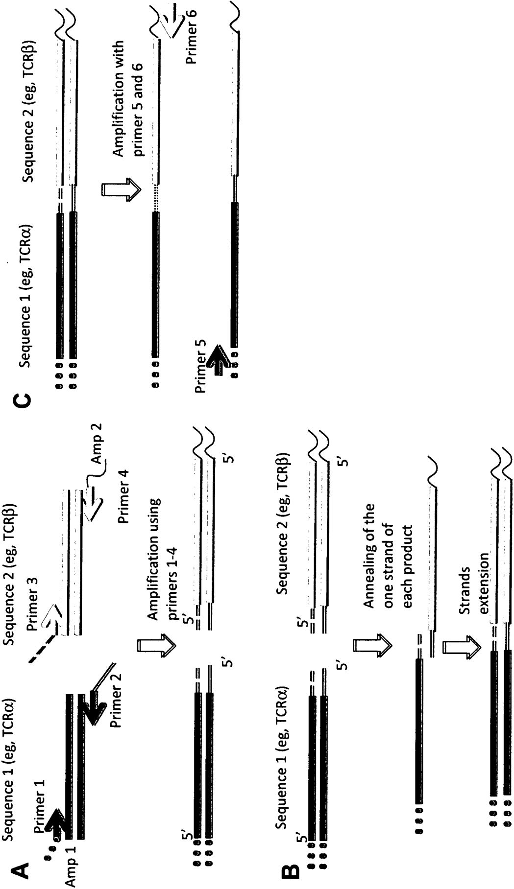
Scheme 2
