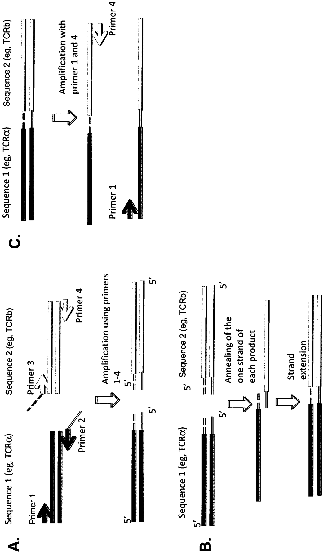
Scheme 1
