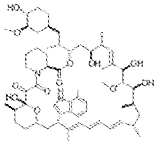
Scheme 1. Structure of AP21967
