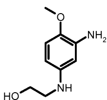
(VII) molare Masse = 182,22 g/mol
