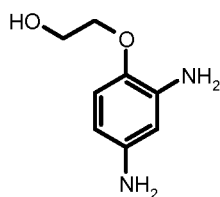
(VI) molare Masse = 168,20 g/mol
