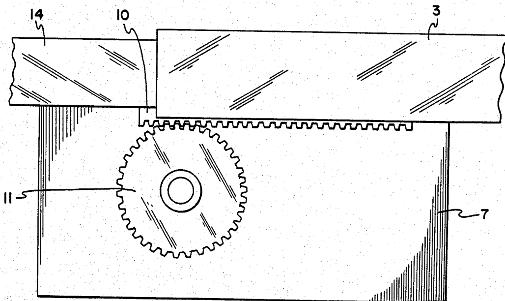
VIEW "Q"
