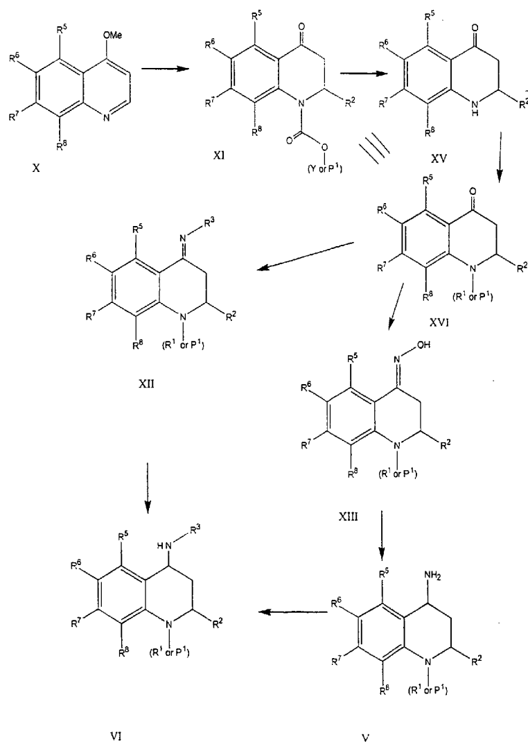
SCHEME II
