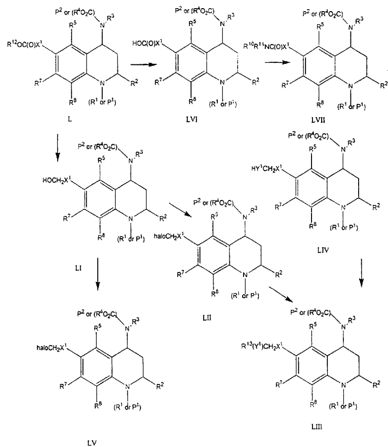
SCHEME V
