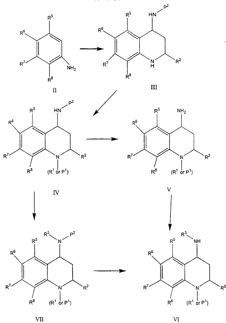
SCHEME I
