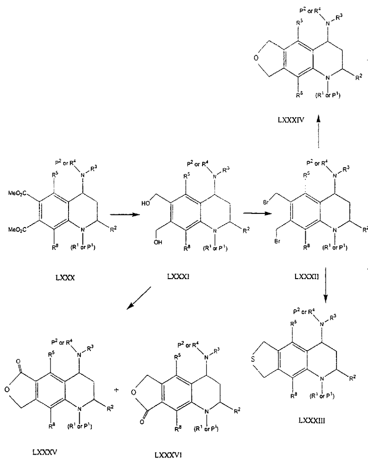
SCHEME VIII
