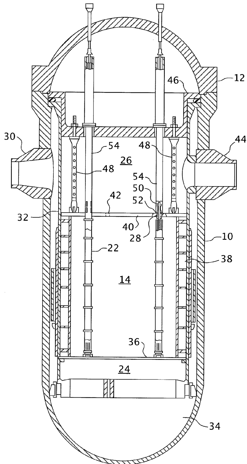
FIG. 2 Prior Art
