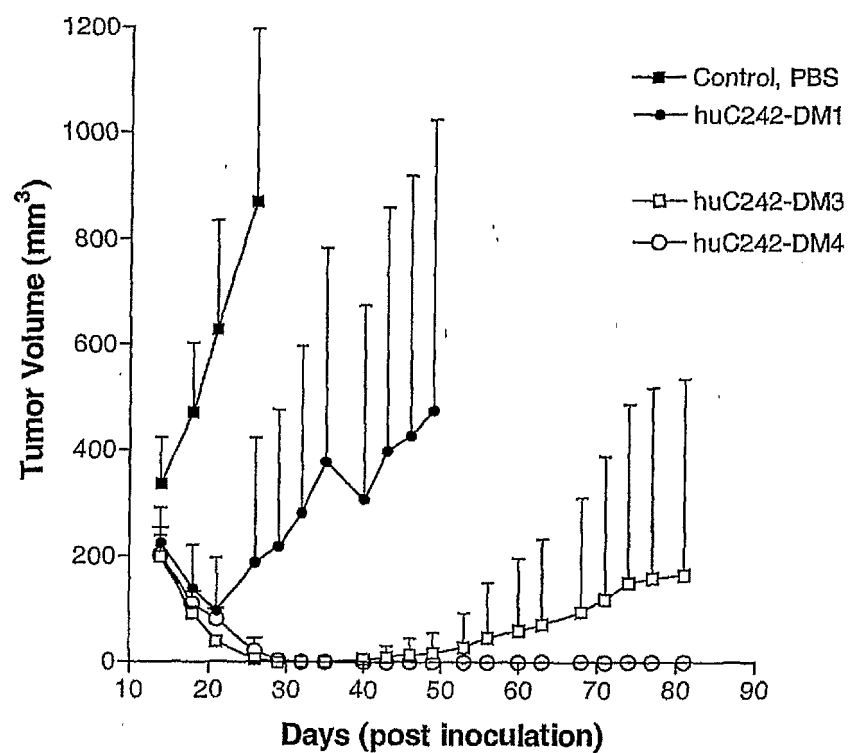
FIG. 8 In vivo Efficacy of huC242-Maytansinoid Conjugates (COLO-205 Xenografts)
