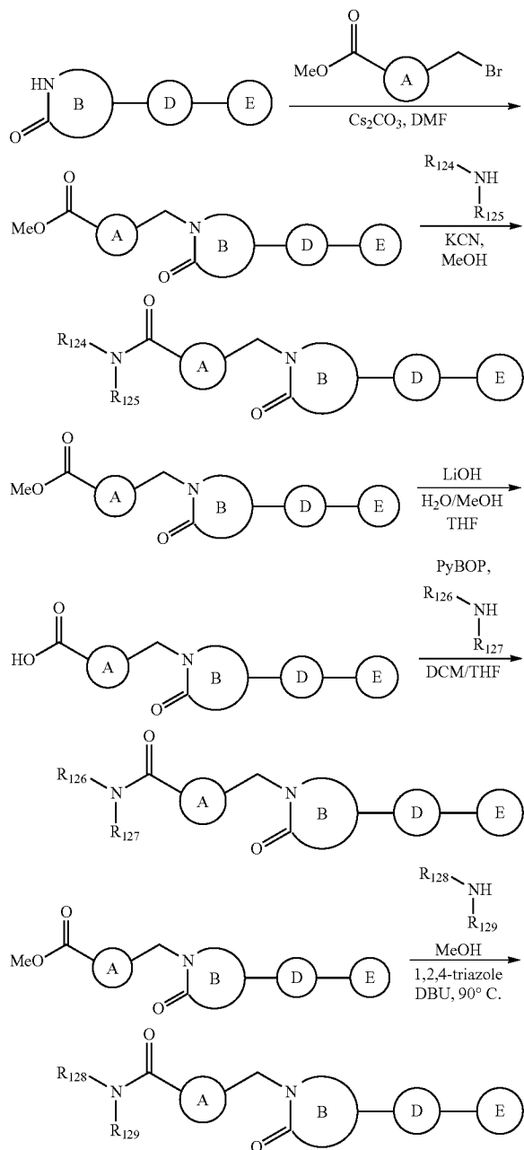
SCHEME 12:
