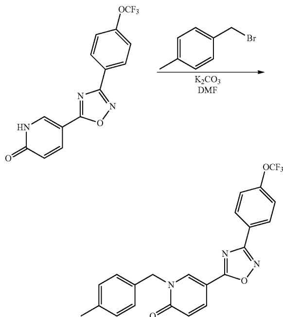
1-(4-Methylbenzyl)-5-(3-(4-(trifluoromethoxy)phenyl)-1,2,4-oxadiazol-5-yl)pyridin-2(1H)-one
