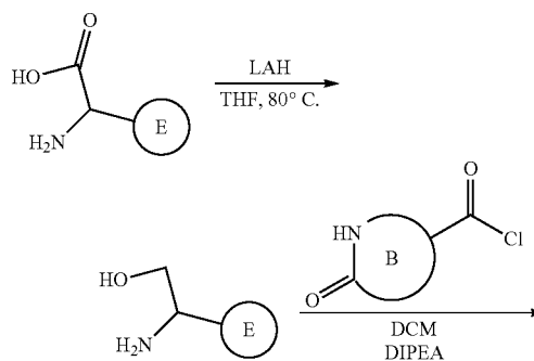
Scheme 16b
