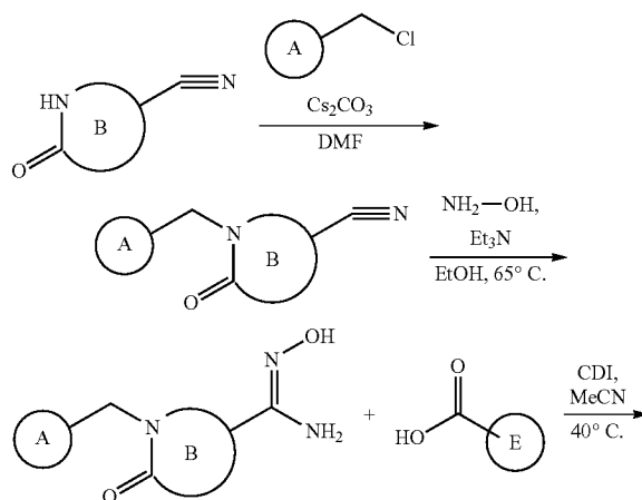
SCHEME 14:
