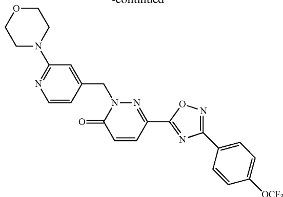
2-((2-Morpholinopyridin-4-yl)methyl)-6-(3-(4-(trifluoromethoxy)phenyl)-1,2,4-oxadiazol-5-yl)pyridazin-3(2H)-one
