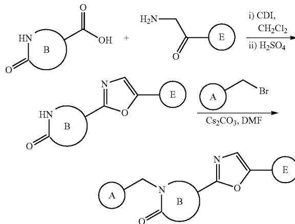
Scheme 16a
