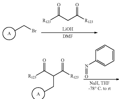
SCHEME 11:
