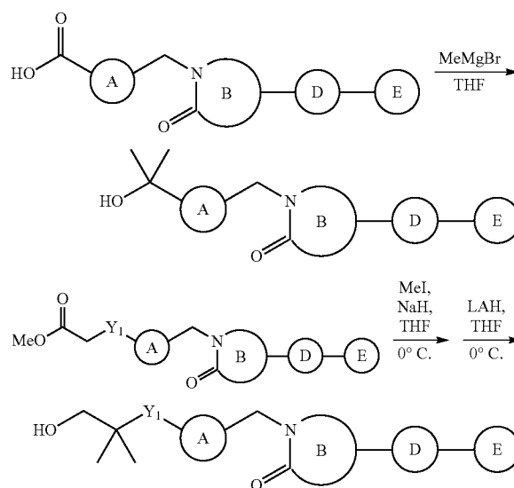
SCHEME 13:
