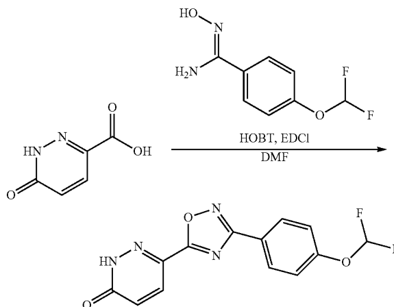
6-(3-(4-(Difluoromethoxy)phenyl)-1,2,4-oxadiazol-5-yl)pyridazin-3(2H)-one
