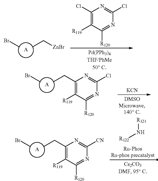
SCHEME 10:
