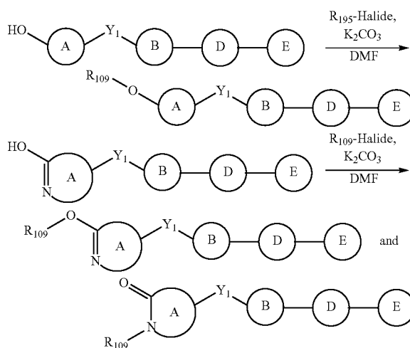
Scheme 7a
