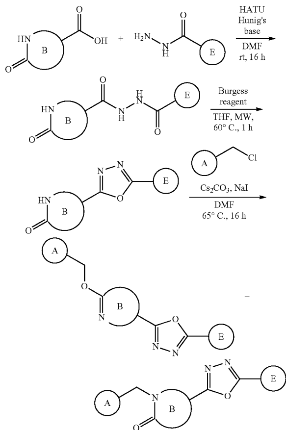
SCHEME 15:
