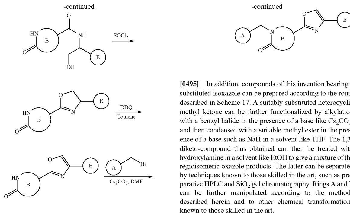
SCHEME 17:
