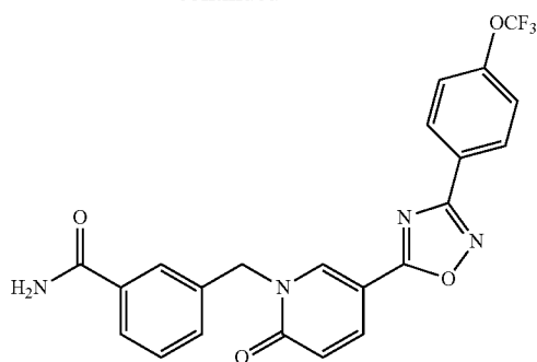
3-((2-oxo-5-(3-(4-(trifluoromethoxy)phenyl)-1,2,4-oxadiazol-5-yl)pyridin-1(2H)-yl)methyl)benzamide
