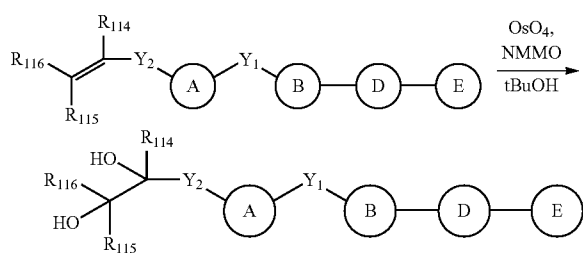
SCHEME 9:
